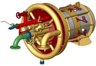
Dual fuel hydrogen and natural gas burner
