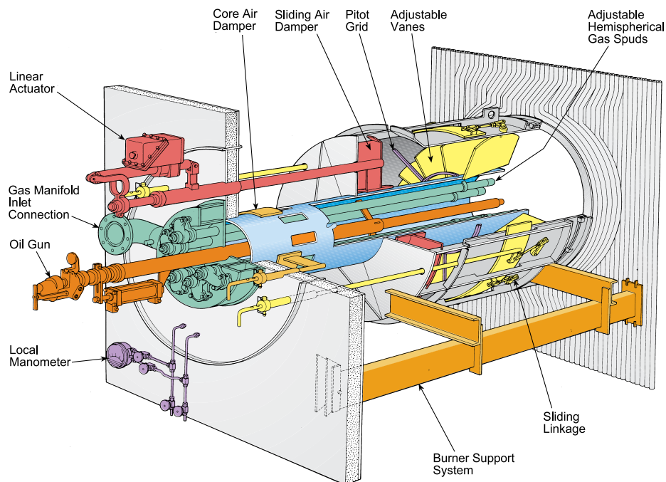
B&W PGG's plug-in type low NO x XCL-S® burner for superior combustion.
