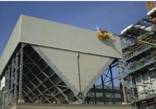
V-Frame design
