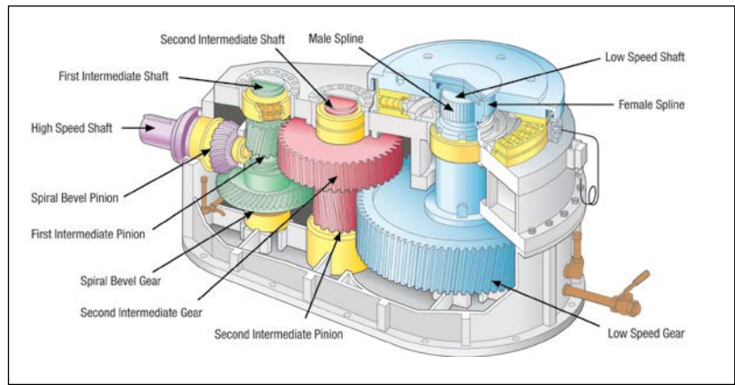
Triple Reduction Gear Drive
