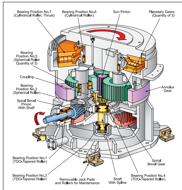
Planetary Gear Drive
