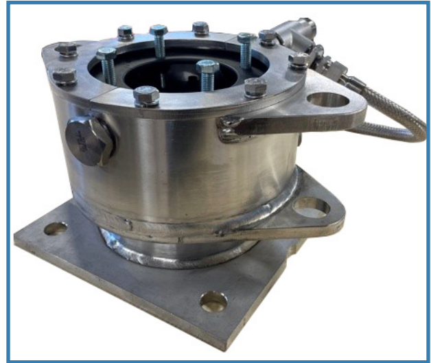
B&W's Diamond Power stainless steel AISI 316L sootblower wallbox is ideal for areas of extensive corrosion.
