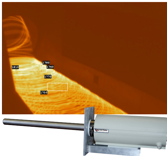
SteelCam® high-resolution camera with TempVu® software system screenshot.
